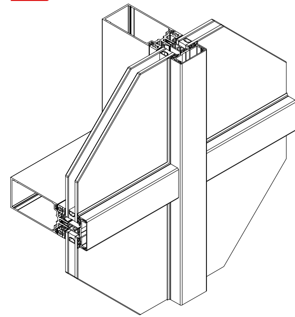
ISOMETRIC VIEW
