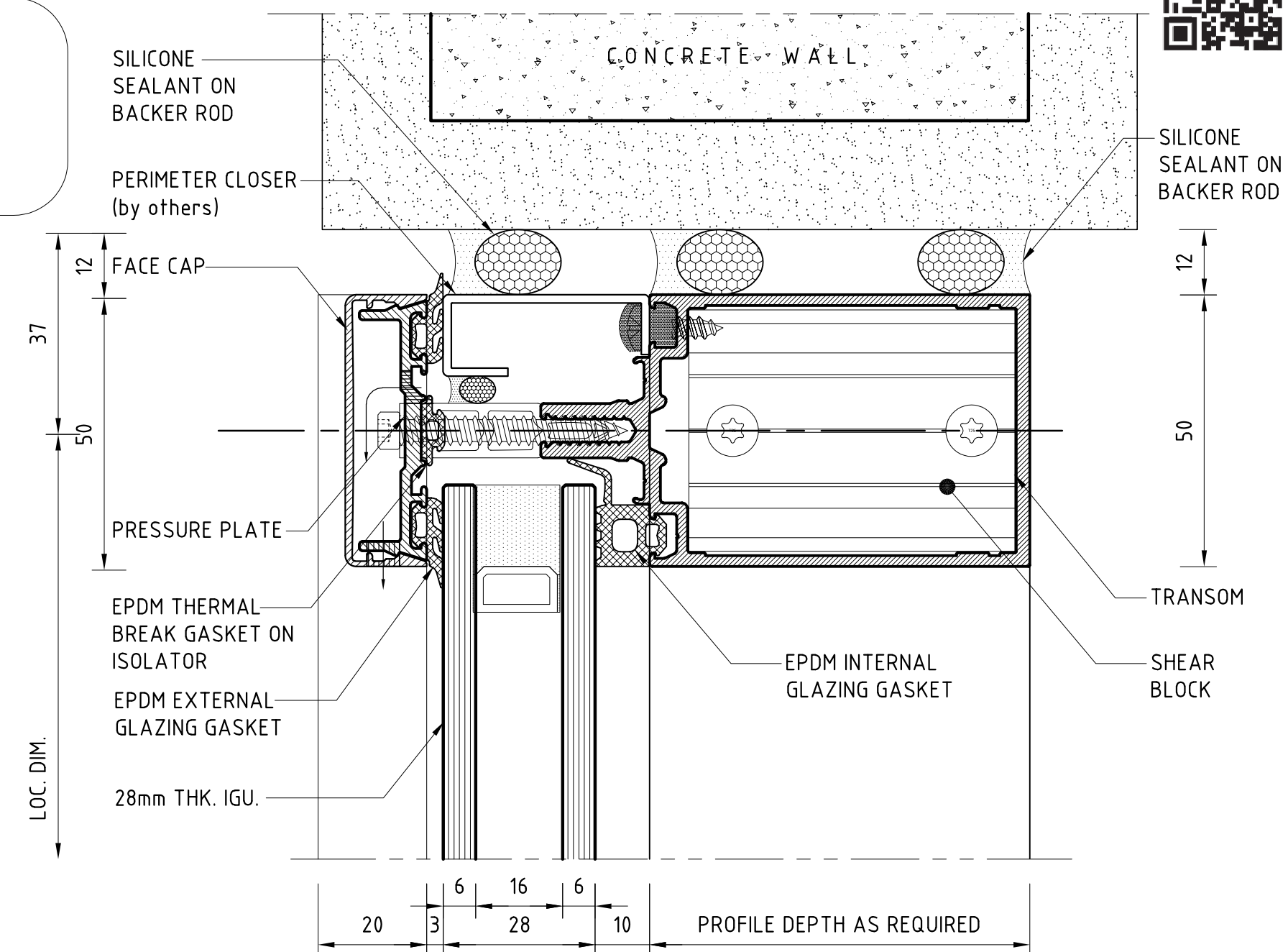
HEAD TRANSOM DETAIL
