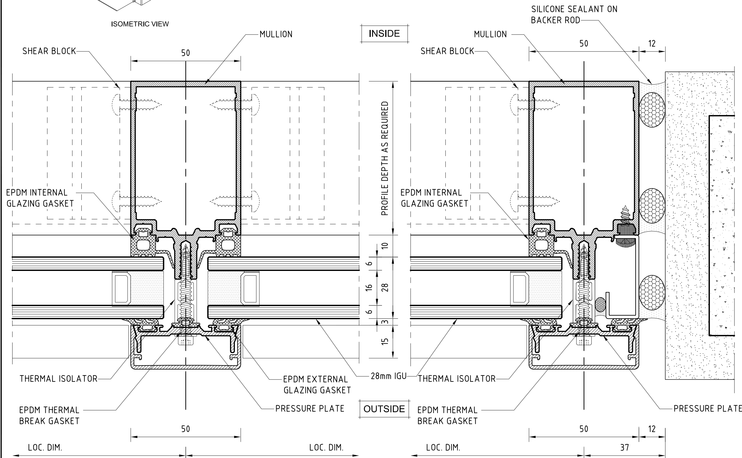
INTERMEDIATE MULLION DETAIL
