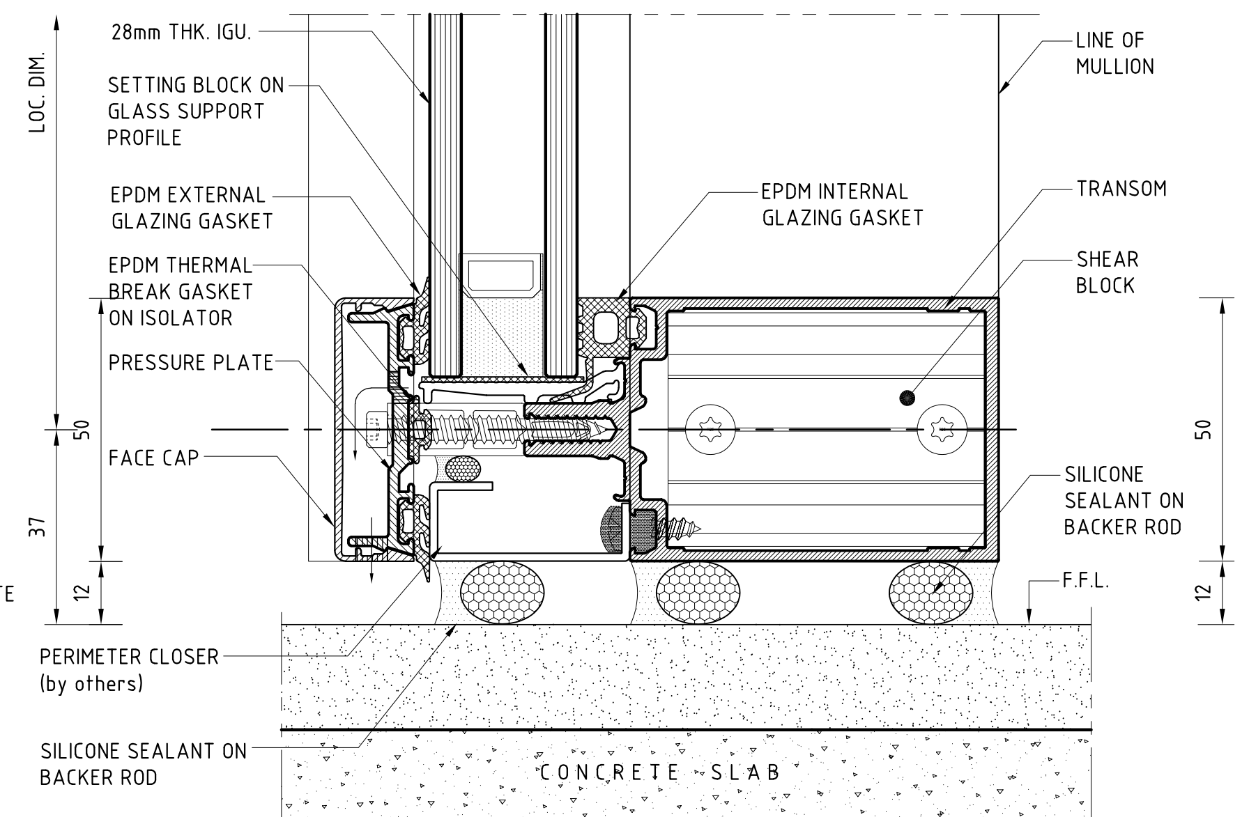
SILL TRANSOM DETAIL
